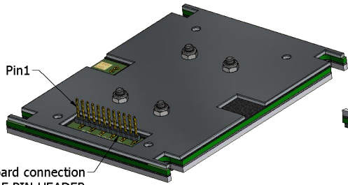
J1 Keyboard connection MALE PIN HEADER 12 pins - 2,54 mm pitch
