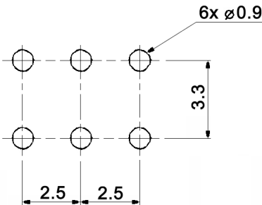
HOLE LAYOUT TOP VIEW
