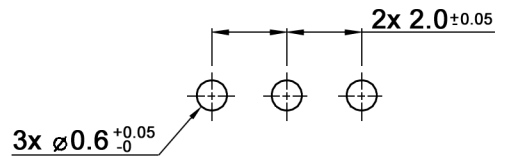
HOLE LAYOUT TOP VIEW \oplus 0.05
