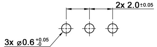
HOLE LAYOUT TOP VIEW \oplus 0.05
