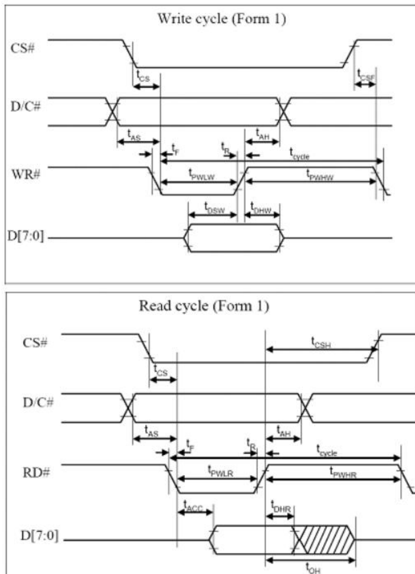
8080-series parallel interface characteristics (Form 1)
