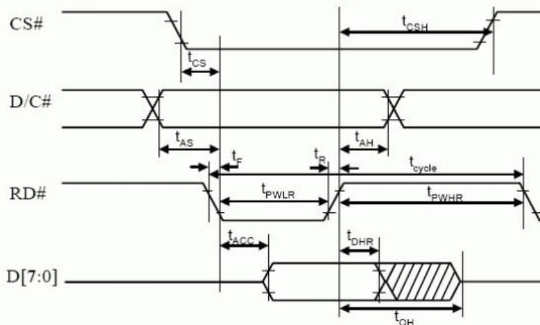
Read Cycle
