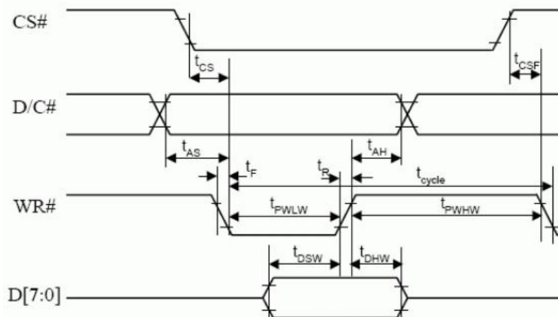
8080-series parallel interface characteristics Write cycle
